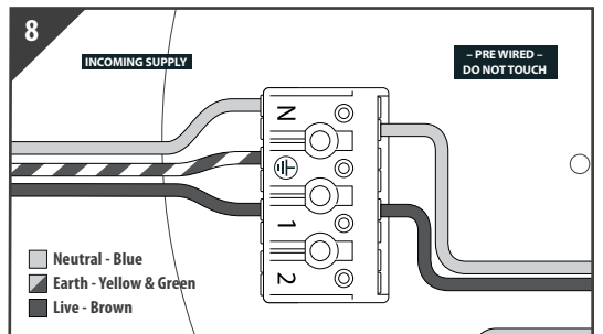
8 Press the individual terminal and insert the correct incoming supply before releasing the terminal to secure. The product MUST be earthed
