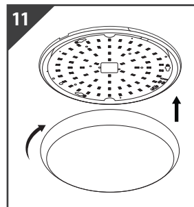
11 Push and twist the diffuser back into place
