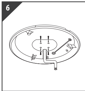
6 Install the fixing screws to the base plate
